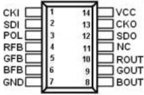
Fig1. SOP-14 package
