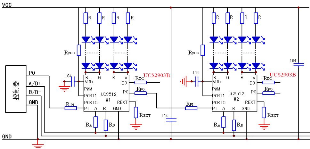
应用图 3: RG, BW 2 字段应用 Application Figure 3: RG, BW 2 field mode application
