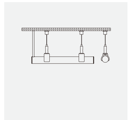
ND25 -“-” type hanging mounting with open PC clips (ND25-IA03)
