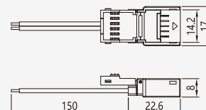
14mm Quick Connector
