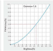
Dimming curve for RGB/DIM
