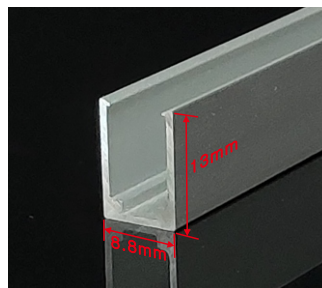
Mounting clip(length: 2cm)
